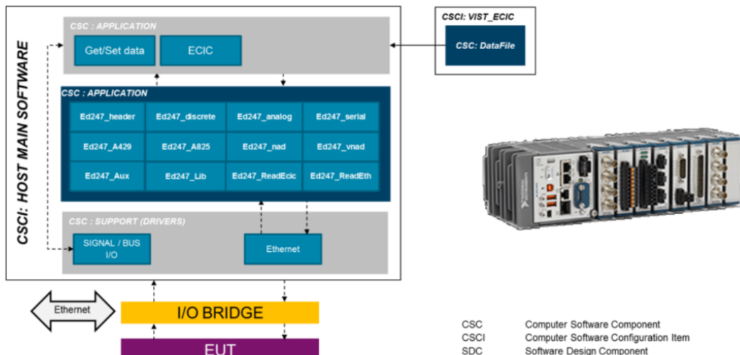
Fig. 5. SW components diagram.
