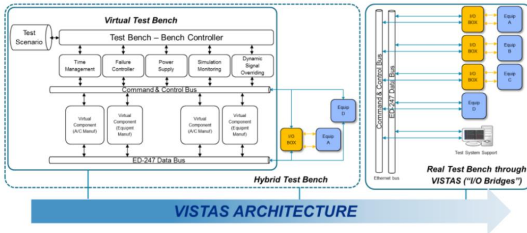
Fig. 2. VISTAS Architecture.
