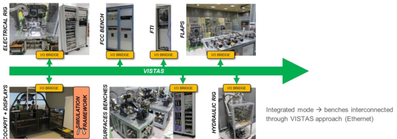
Fig. 4. Cleansky 2 Integrated Rig with VISTAS protocol implemented.
