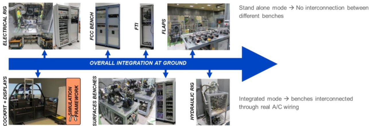
Fig. 3. Cleansky 2 Integrated Rig.
